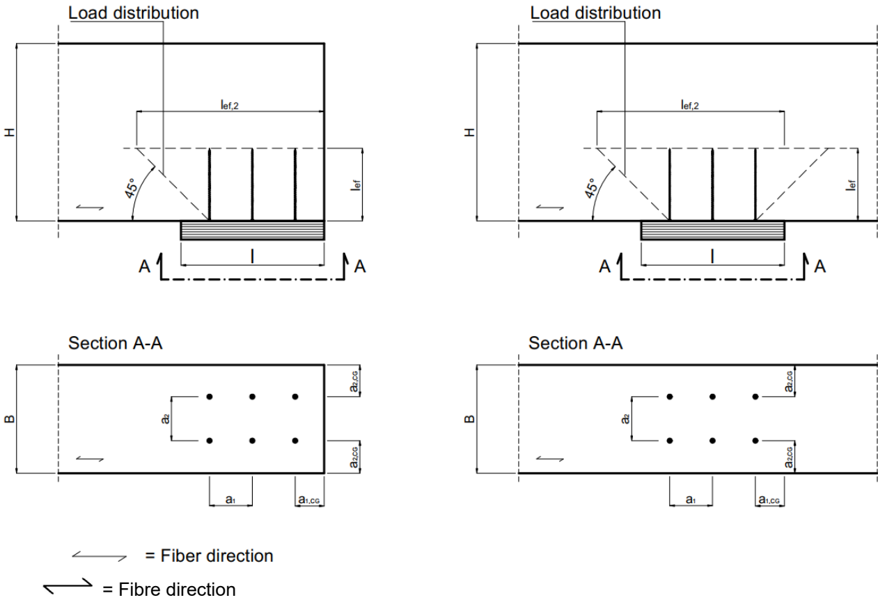
Figure A.3.1 Reinforced end support (left) and reinforced intermediate support (right)
